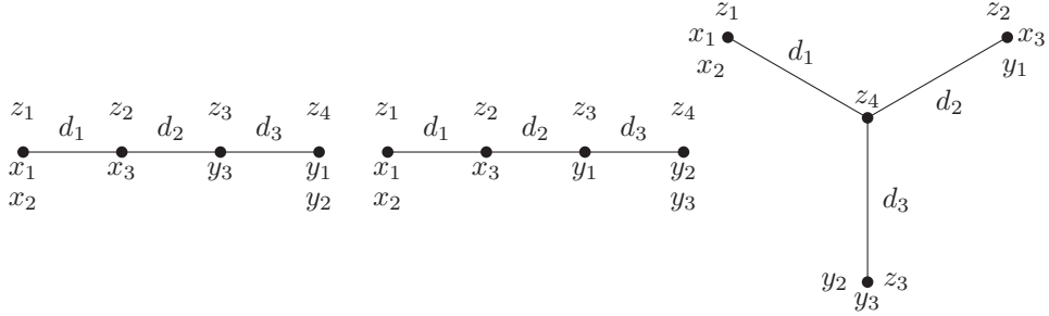
Figure 3: Possible stable limits of T
